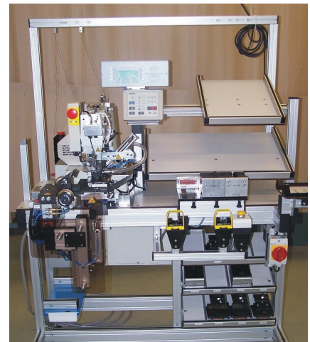
End bracket-Line
