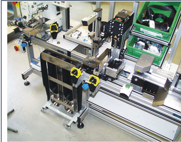
Pin- and Retractor Feeder
